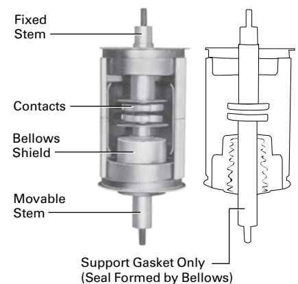
Cut-Away View of Vacuum Interrupter (Enlarged to Show Detail)
