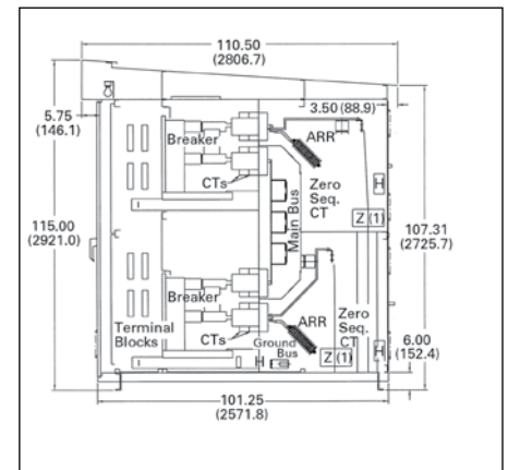
Figure 5.1-31. Outdoor Aisleless
