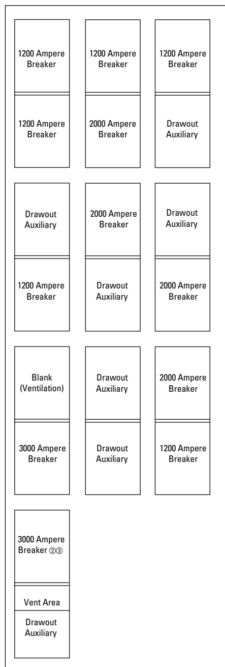
Figure 5.1-24. Available Configurations
