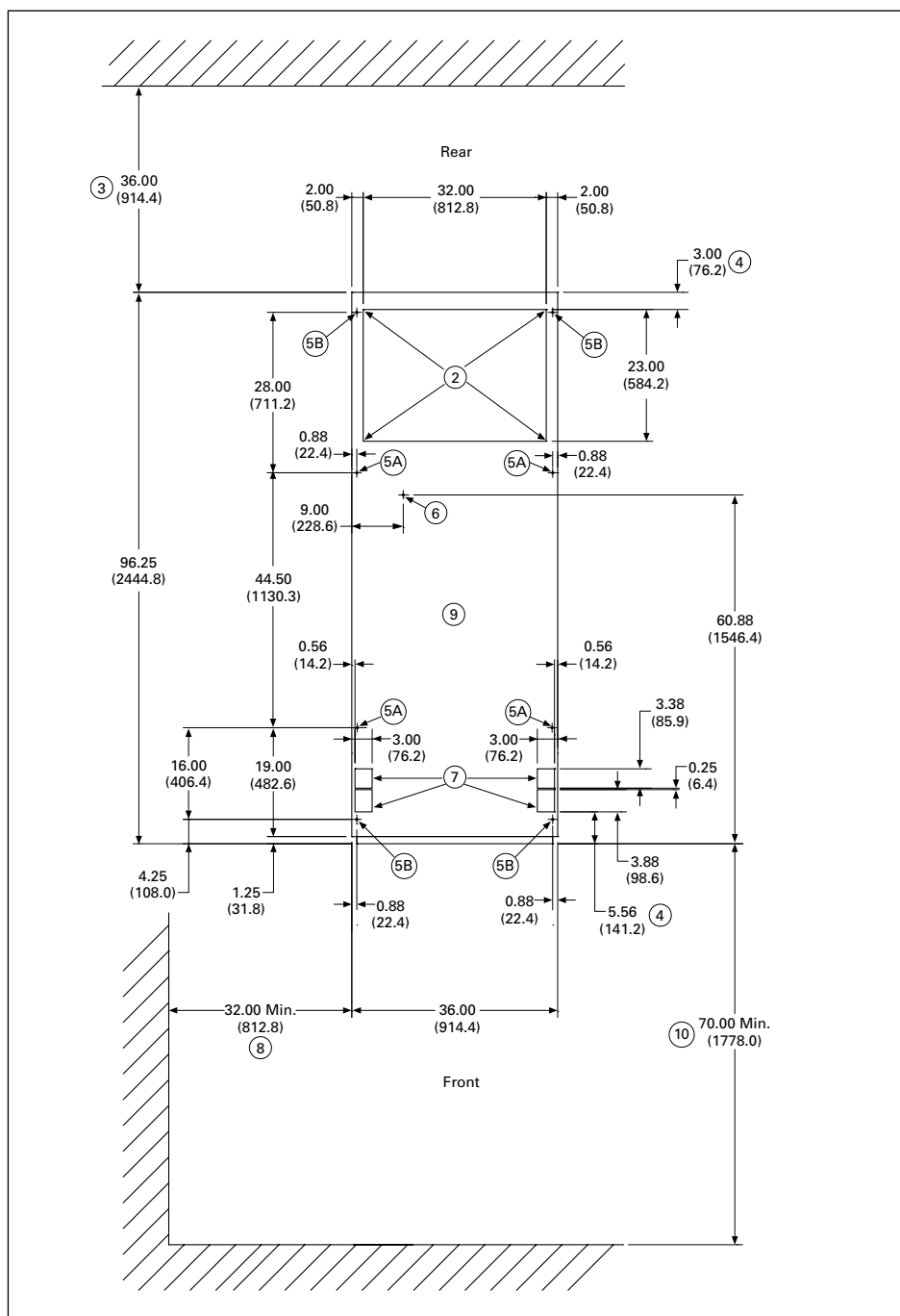
Figure 5.1-33. Base Plan of a Typical Indoor Breaker or Auxiliary Structure
