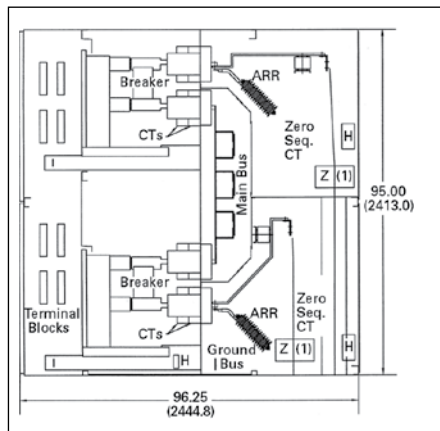
Figure 5.1-30. Indoor
