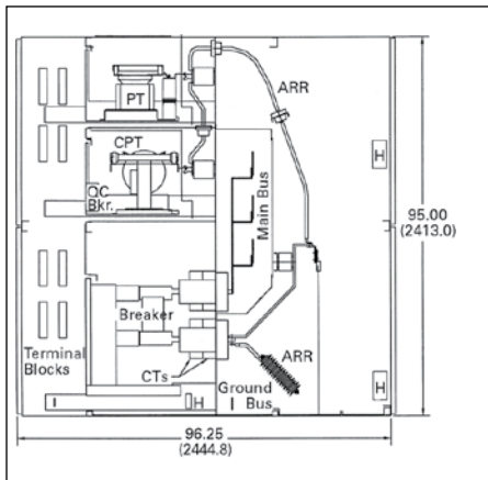
Figure 5.1-26. 36.00-Inch (914.4 mm) Wide Typical Auxiliary/Breaker Vertical Section
