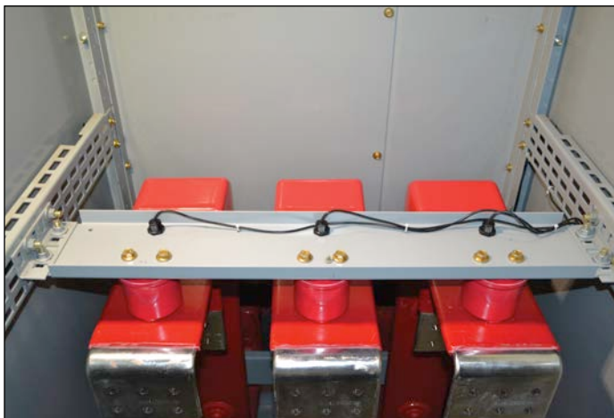
Figure 5.1-10. Typical Install for Continuous Thermal Monitoring Sensors
